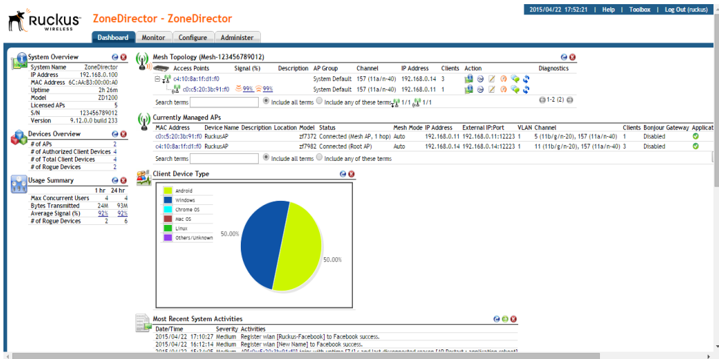
Figure 12. The Dashboard
