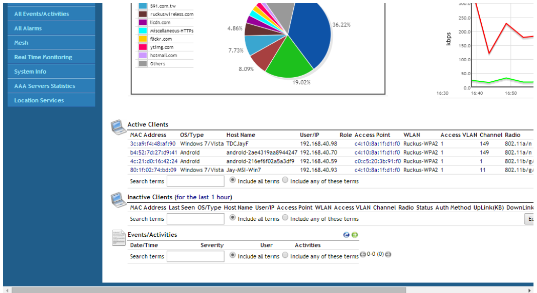
Figure 177. Monitoring Clients
