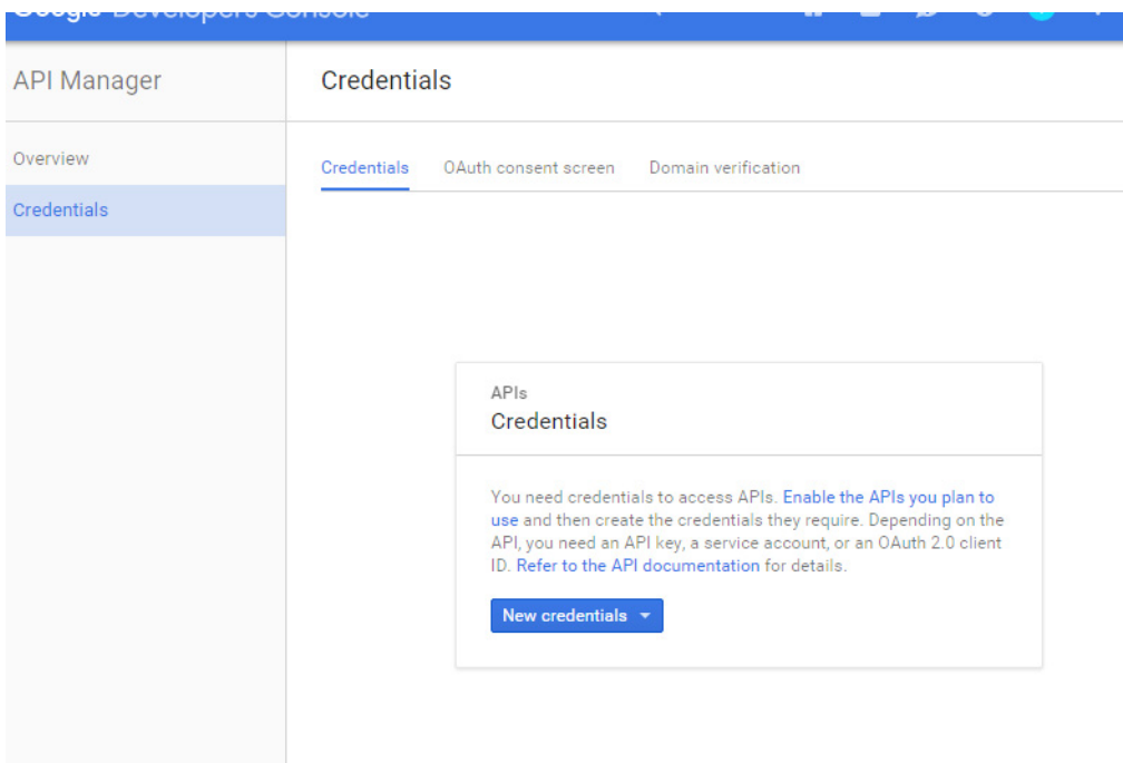
Figure 115. Credentials page
